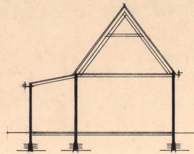
DWARSKNED.
