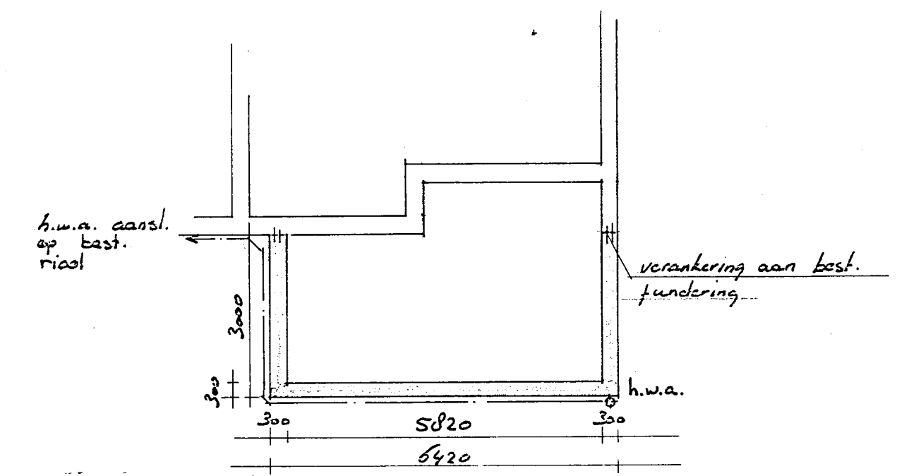
Fundering / Ruitering
