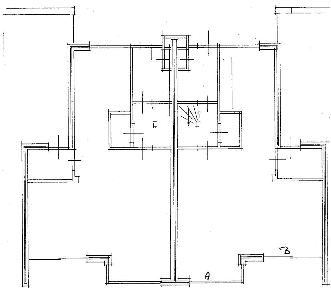
Best. Begane-Grond
