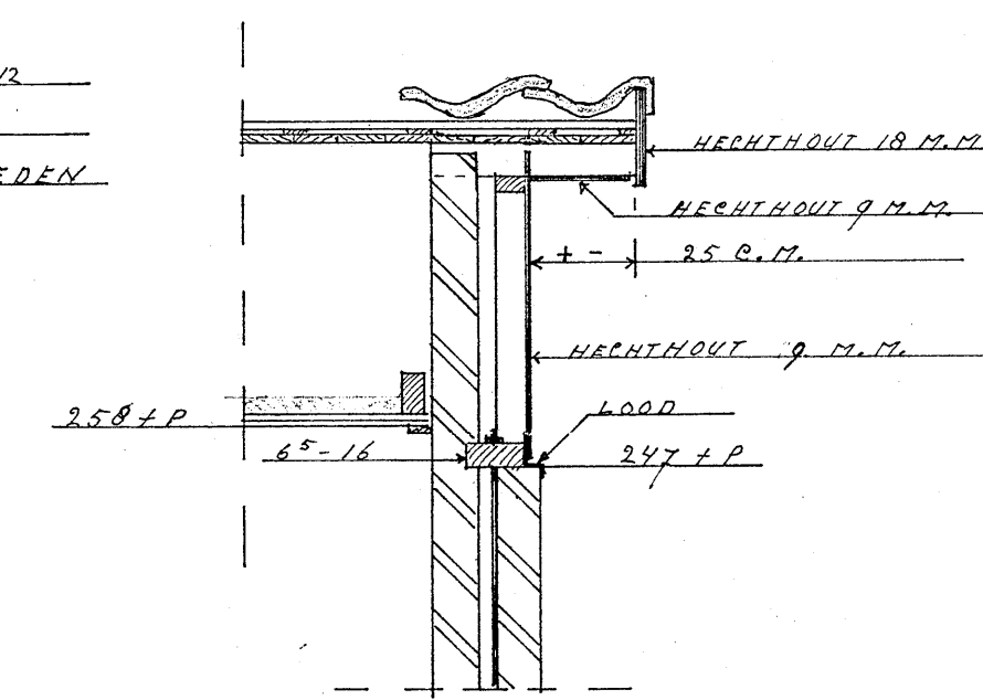
detail - B
