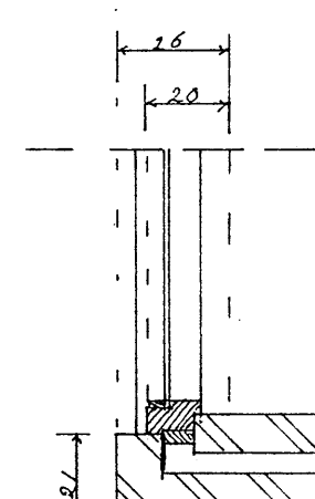
detail - D
