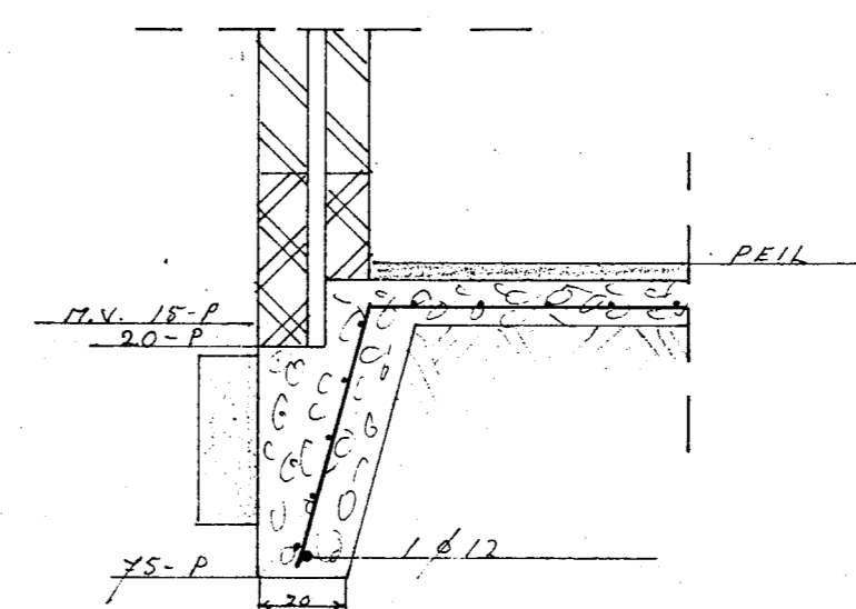
detail - D
