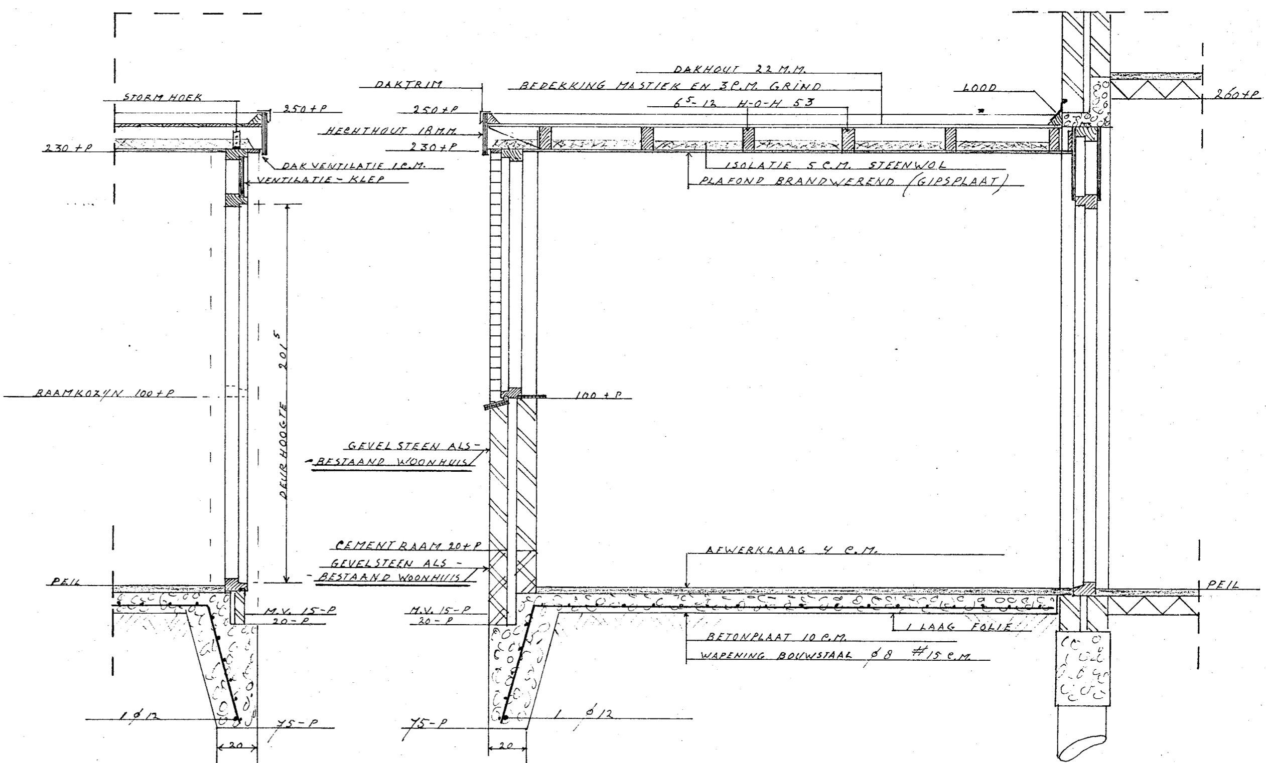
detail - B
