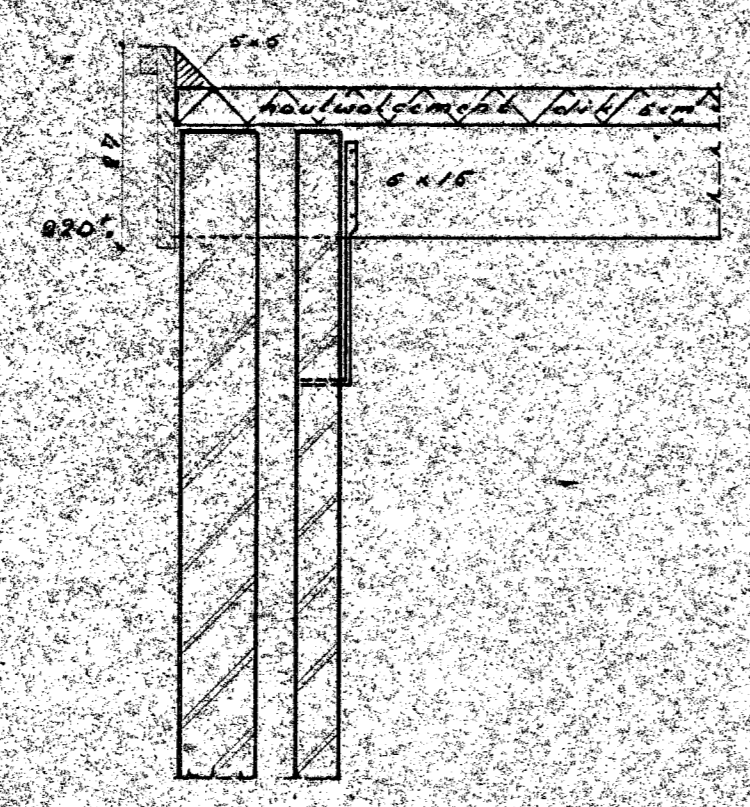
dakdetail
