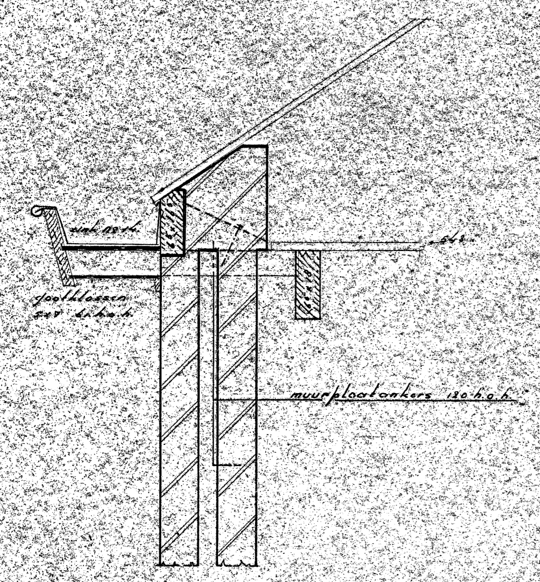
gootdetail
