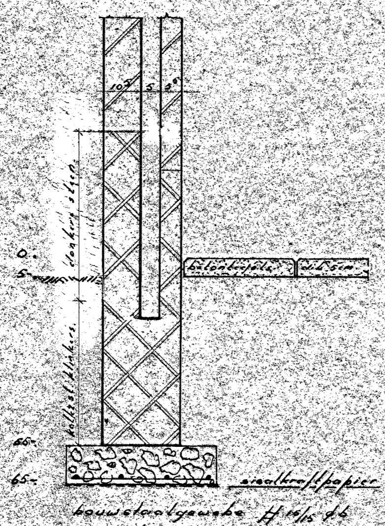
fundering detail garage
