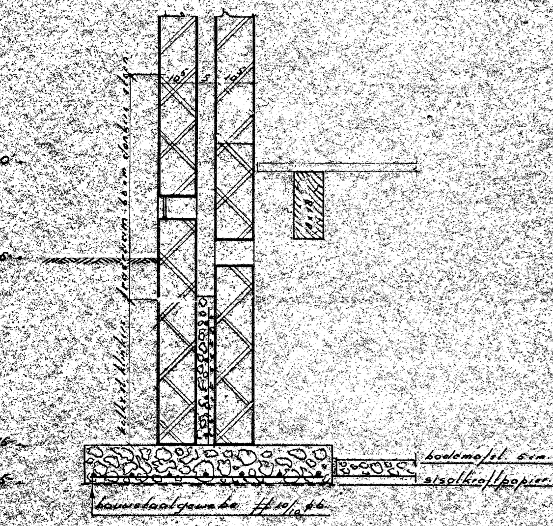
fundering detail woning
