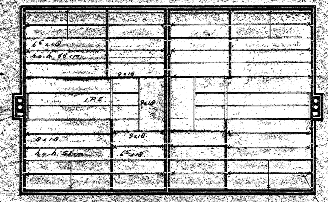
zolder balklaag
