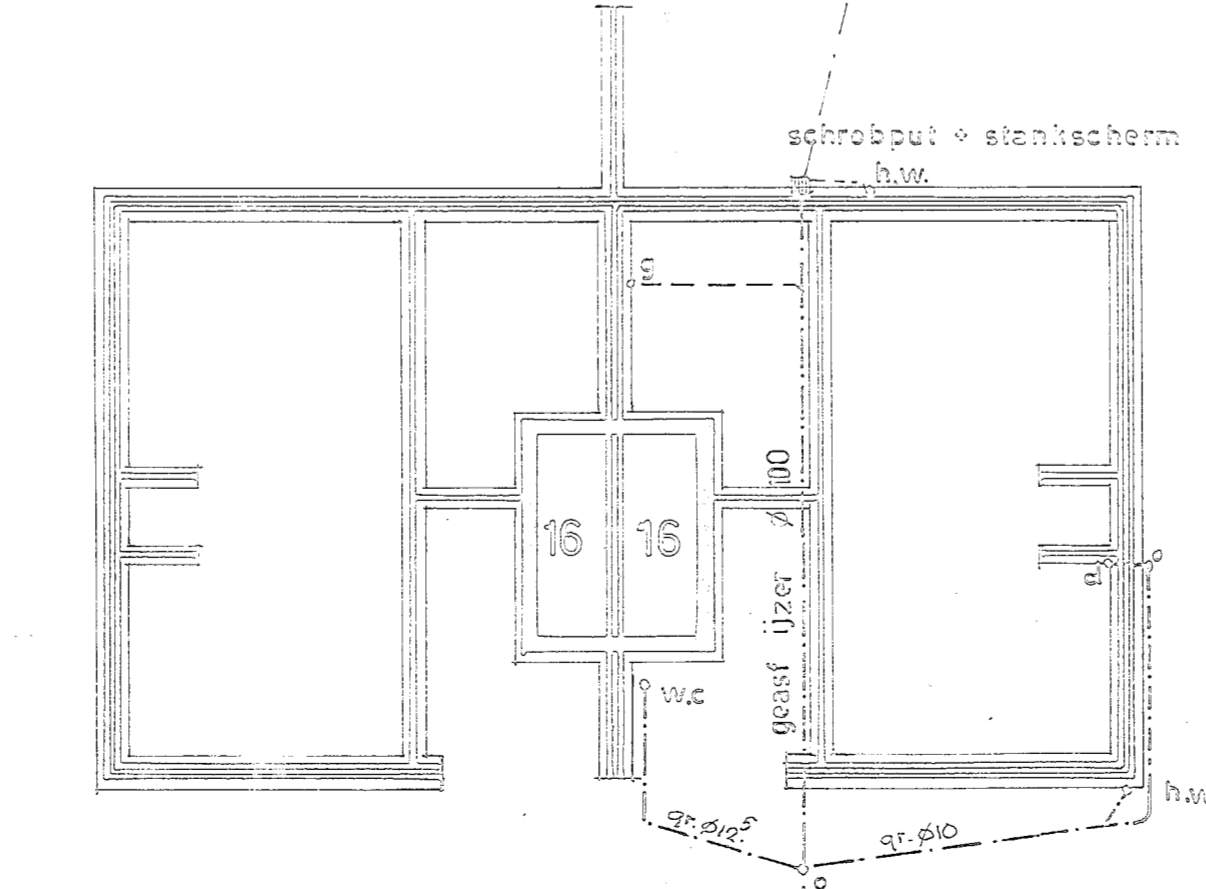
FUNDERING RIOLERING
